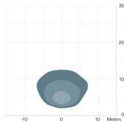
1010 Flush / 700 lm Wide 45°+ 3.0 m / -15° Symmetric
