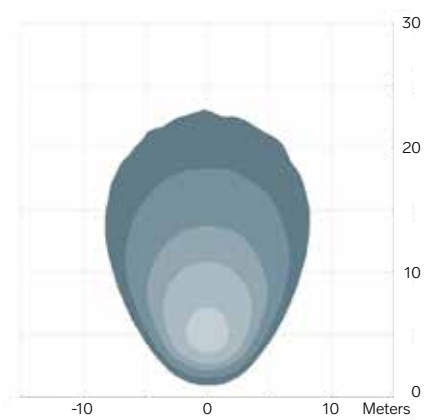
1010 Swivel / 2500 lm Medium 31-45° 3.0 m / -15° Symmetric
