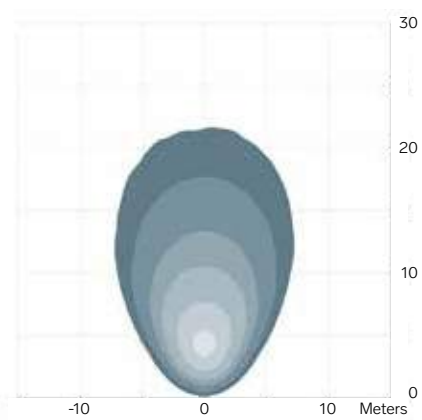
1010 Swivel / 2500 lm Medium 31-45° 3.0 m / -15° Asymmetric
