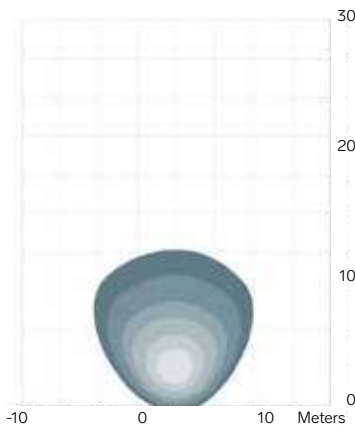
1313 AC / 3700 lm Wide 45°+ 3.0 m / -15° Asymmetric
