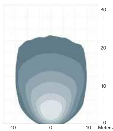
1323 / 13,500 lm Wide 45°+ 3.0 m / -15° Symmetric
