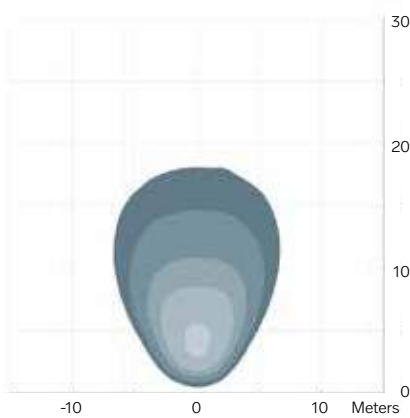
1010 Recess / 1450 lm Medium 31-45° 3.0 m / -15° Symmetric
