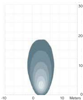
1313 AC / 3700 lm Wide 45°+ 3.0 m / -15° Symmetric
