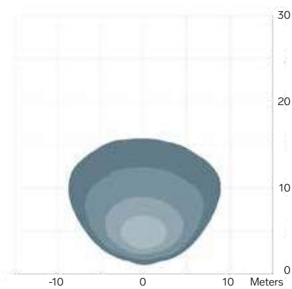
1010 Recess / 1450 lm Wide 45°+ 3.0 m / -15° Symmetric
