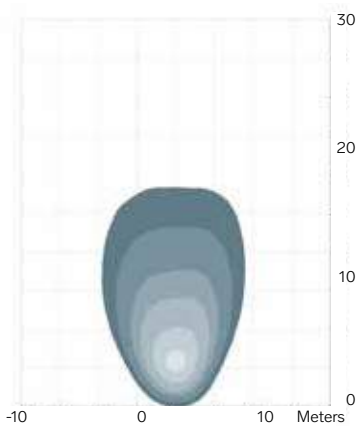
1313 AC / 3700 lm Medium 31-45° 3.0 m / -15° Symmetric
