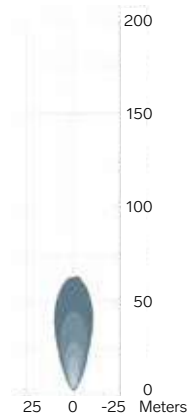
1010 Flush / 700 lm High 1.0 m / 0° Symmetric
