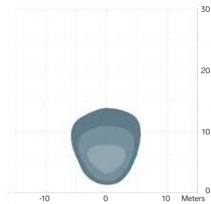
VL6 / 1000 lm Wide 45°+ Symmetrical
