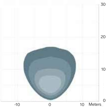
1010 Recess / 1450 lm Wide 45°+ 3.0 m / -15° Asymmetric
