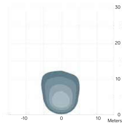
VL6 / 1000 lm Wide 45°+ Asymmetrical
