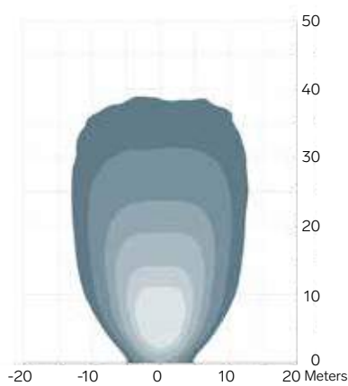
1323 / 13,500 lm Medium 31-45° 3.0 m / -15° Symmetric
