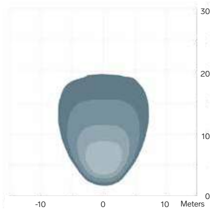
1010 Recess / 1450 lm Narrow 0-30° 3.0 m / -15° Symmetric
