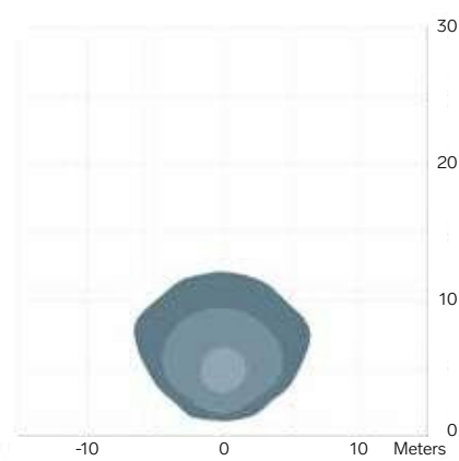
0606 / 720 lm Wide 45°+ 3.0 m / -15° Symmetric
