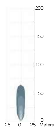
0606 / 750 lm Spot 1.0 m / 0° Symmetric
